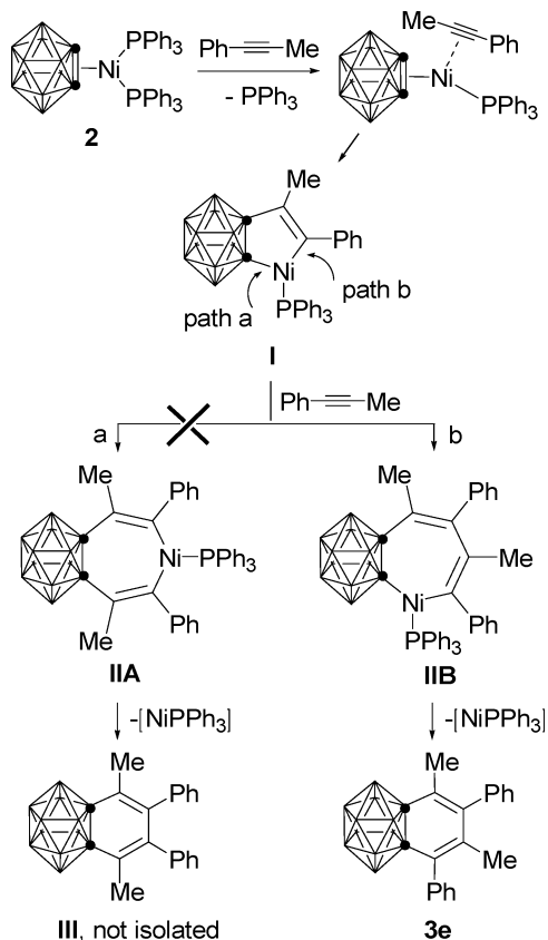
Scheme 1. Proposed Mechanism for the Formation of 3e
